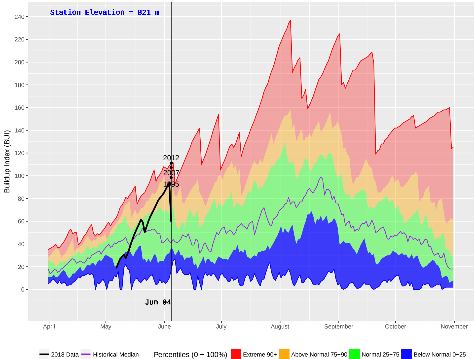
KNIFE (225) : Historical (1991–2016) and Current (2018) Noon Buildup Index (BUI)
