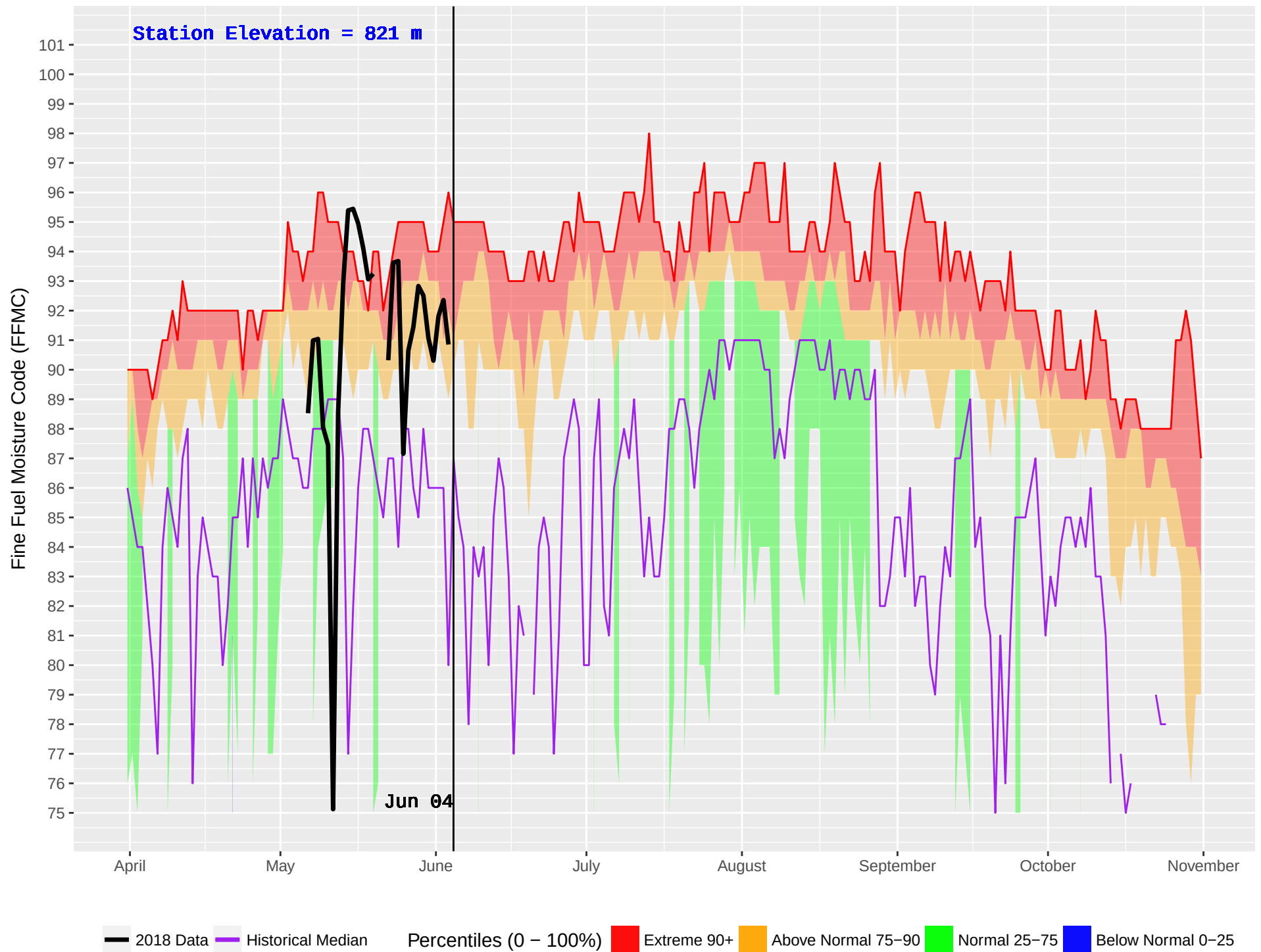
KNIFE (225) : Historical (1991–2016) and Current (2018) Noon Fine Fuel Moisture Code (FFMC)
