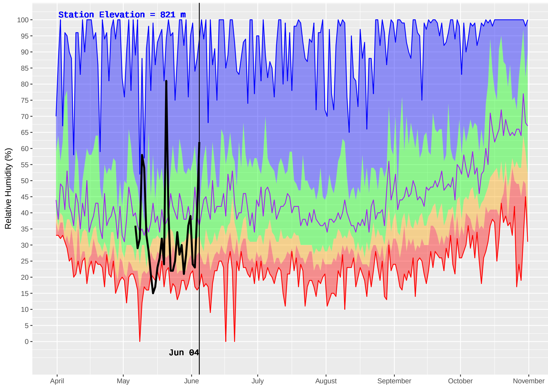
KNIFE (225) : Historical (1991–2016) and Current (2018) Noon Relative Humidity
