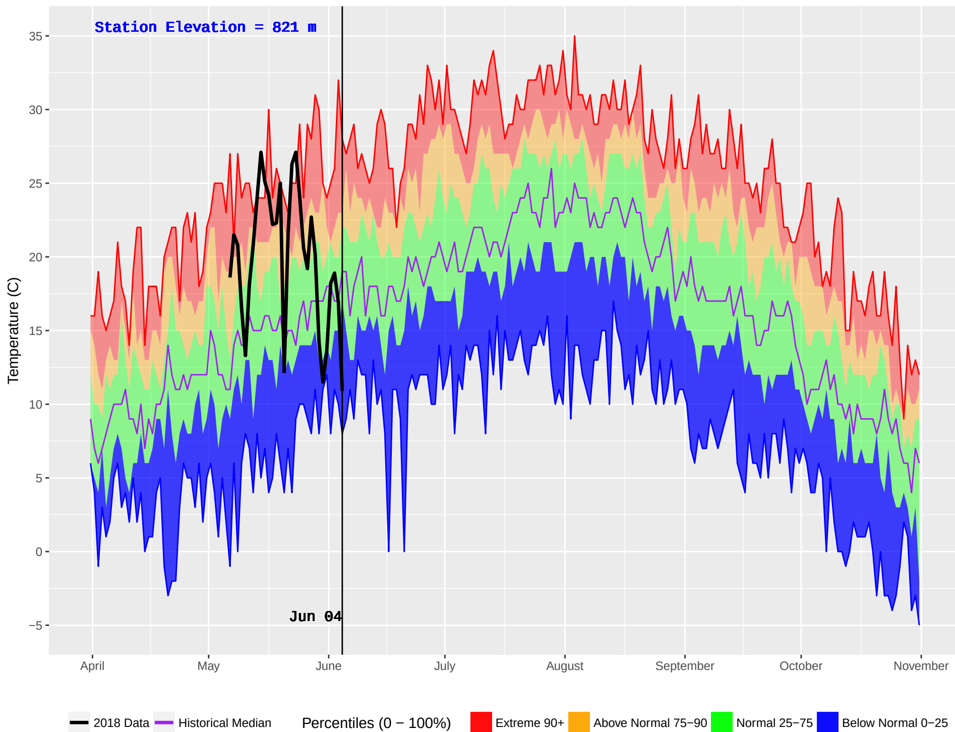
KNIFE (225) : Historical (1991–2016) and Current (2018) Noon Temperature
